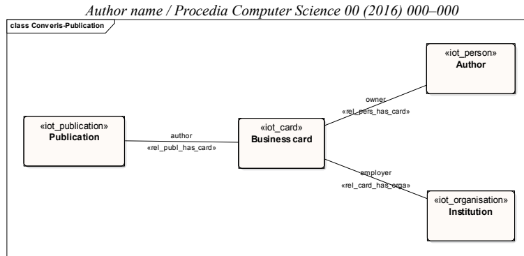
Figure 4. A class diagram depicting the relevant Converis entities and relations involved in the description of authorship and affiliations.
