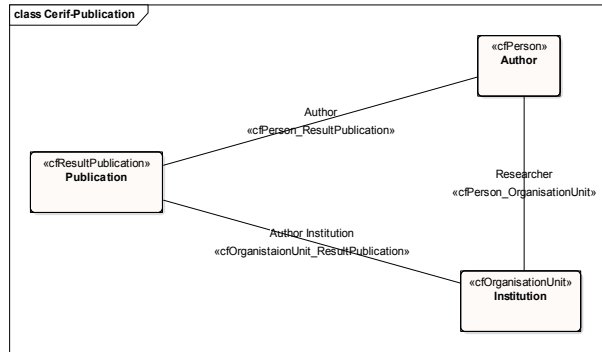
Figure 2. A class diagram showing the relations between Publications, Authors and their Institutions as they are described in standard CERIF.
