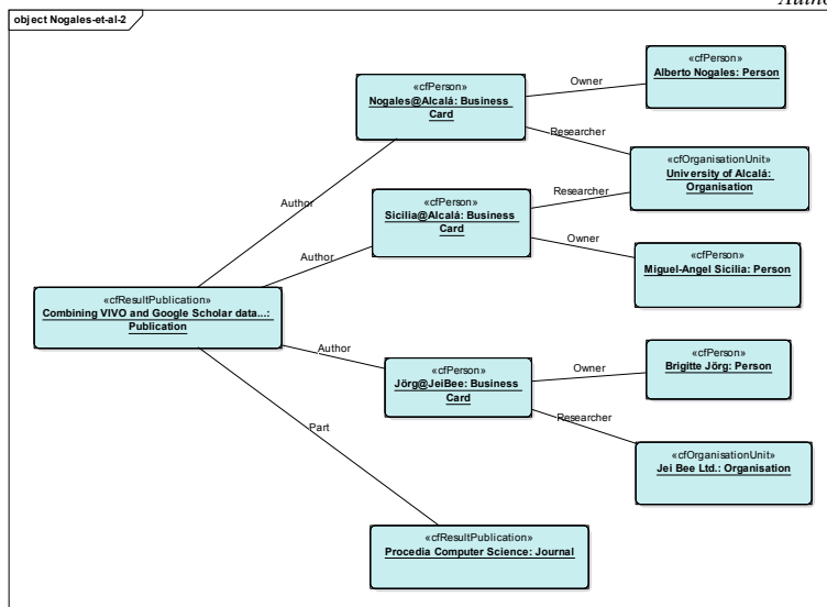
Figure 6. An object diagram modeling the publication in Figure 1 in the proposed schema.
