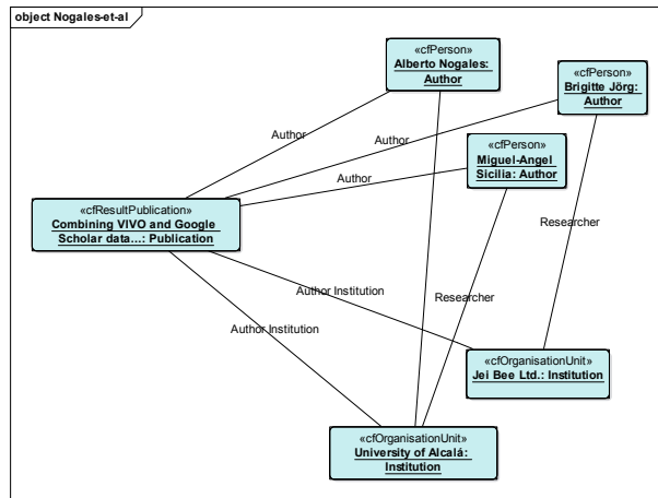
Figure 3. An object diagram showing the affiliation information in Figure 1 represented in standard CERIF.
