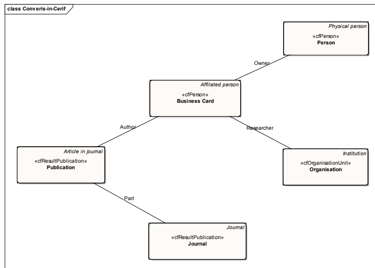
Figure 5. A class diagram showing the proposed extension of the standard way of modelling authorship and affiliations in CERIF.
