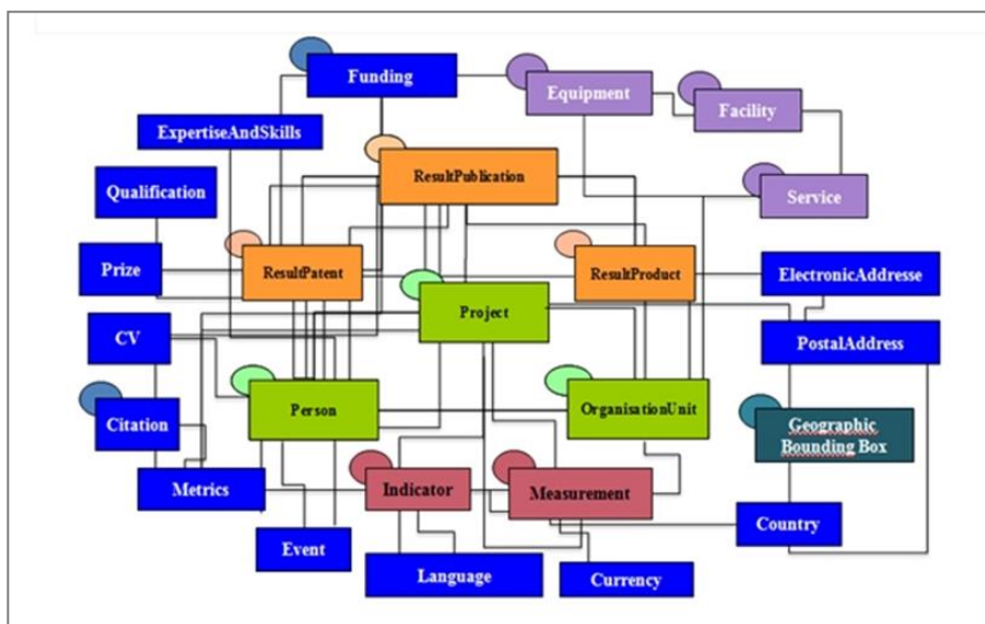
Figure 1: Overview of the CERIF 1.6 E-R model. Research information is modelled in base entities (green), result entities (orange), infrastructure entities (purple) and so-called second level entities (blue) that represent the contextual environment around the base and result entities. All entities are linked together via time-stamped relations, that are described via link entities or classification references.
