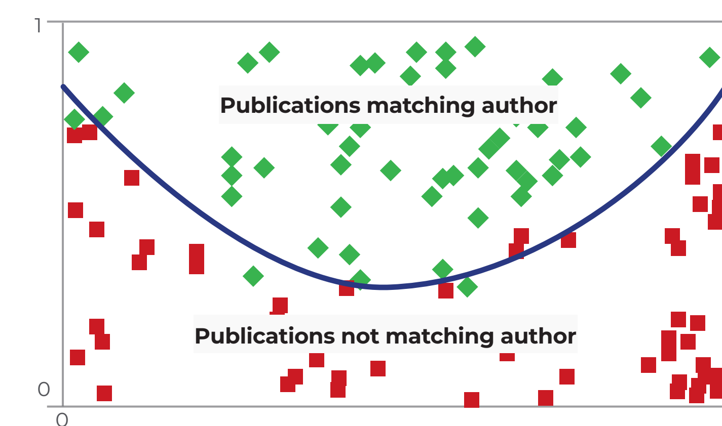
The Author Matching Algorithm
